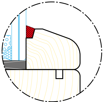
Fermavetro riportato soft Soft attached glazing bead
